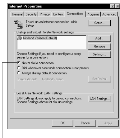
Figure 4-2: Internet properties.
